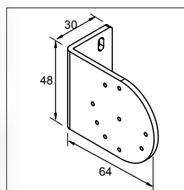
Supporti
